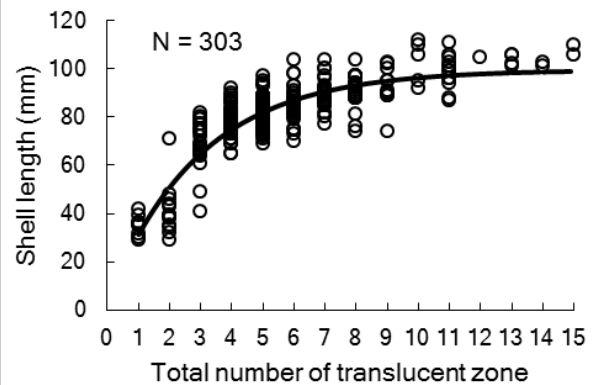
Fig. 5 Relationship between observed current shell length and the total number of translucent zone. The curve shows von Bertalanffy's growth curve of the surf clam. Age = total number of translucent zone \pm 0.5 years old.
