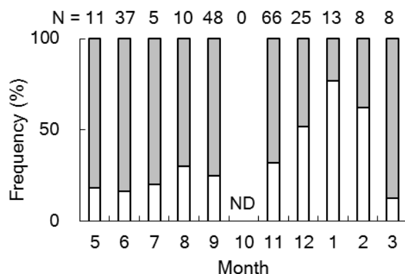
Fig. 3 Seasonal change in the proportion of specimens with translucent and opaque zones on ventral margins of their shell. □, translucent zone; ■, opaque zone.
